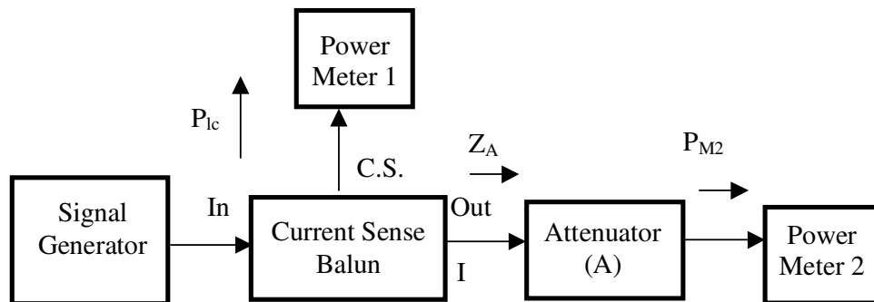
Figure 96: Current Sense Balun, Calibration set-up
